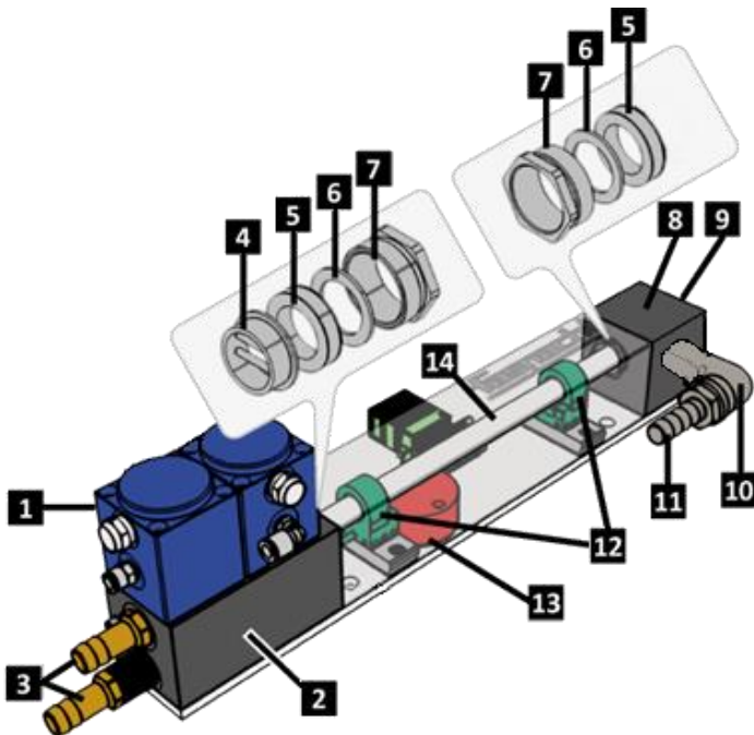
Figure: Viscometer FAS-FB5020, Falling body measuring unit
