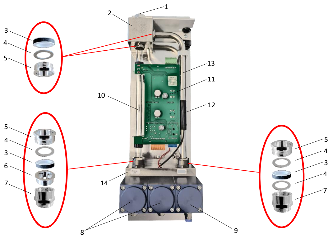
Figure: Viscometer Z3570A
